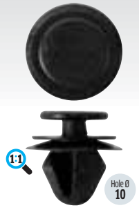
Black Floor Covering Clips Ø x H: 18.5 x 18 mm Part No. Pack of FIX255 50 PSA 699156 Renault 7703077469
