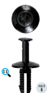
Black Push Rivets Ø x S: 15 x 15 mm Part No. Pack of FIX107 50 BMW 51111908077 Merc A0009905492
