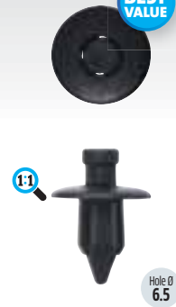
Black Push Rivets Ø x S: 15 x 9 mm Part No. Pack of FIX510 50 GM 96057846 Mitsubishi MB476821 Suzuki 09409073085PK Toyota 9046707041
