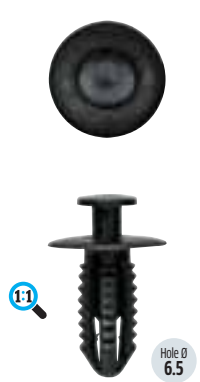
Black Push Rivets Ø x S: 16 x 18 mm Part No. Pack of FIX759 20 Merc A1249900492
