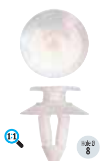
Natural Panel Clips Ø x H: 18 x 21 mm Part No. Pack of FIX80 50 VW 171867299B / 893867290 BMW 51411885961
