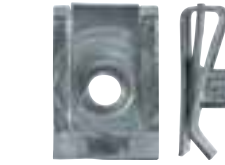
11 Thread Ø: M5 W x L x R: 15 x 21 x 10 mm Part No. Pack of HUC50 25
