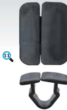
Black Seal Clips W x D x H: 23 x 29 x 15 mm
