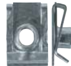
11 Thread Ø: M8 W x L x R: 18.5 x 28 x 14 mm Part No. Pack of HUC58 10
