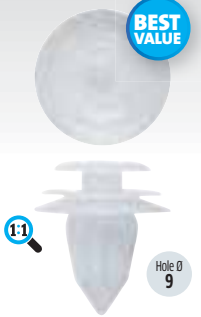
Natural Panel Clips Ø x H: 18 x 20.5 mm Part No. Pack of FIX531 50 GM 909130115 Toyota 9046710161
