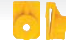
11 Hole Ø: 3 W x L x R: 17 x 12 x 9.5 mm Part No. Pack of FIX409 20 Fiat 1488680
