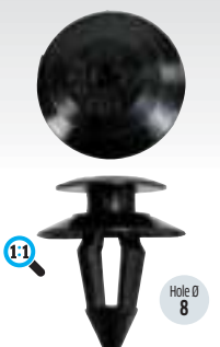
Black Panel Clips Ø x H: 18 x 21 mm Part No. Pack of FIX160 20 VW 703867299
