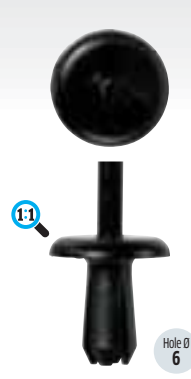
Black Drive Rivets Ø x S: 16 x 14 mm Part No. Pack of FIX175 50 Merc A0009904529 PSA 79030721 / 740760 Volvo 12681763
