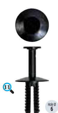
Black Push Rivets Ø x S: 15 x 15 mm Part No. Pack of FIX111 50 VW N90359101 BMW 51111908077 Merc A0009905492 / A0009905492 / A1249900492
