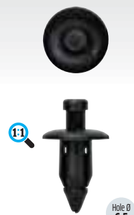
Black Push Rivets Ø x S: 13 x 8 mm Part No. Pack of FIX760 20 Chrysler 6682401G00 Nissan 6682401G00
