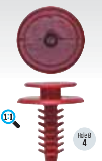
Red Lining Clips Ø x H: 18 x 22 mm Part No. Pack of FIX824 20 Fiat 46410400 / 500358567
